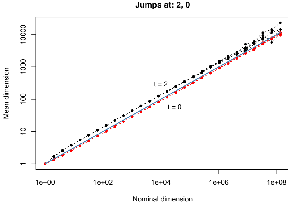
FIG. 2. Computed mean dimension for f(\mathbf{x}) = 1\{\theta^\top \mathbf{x} > t\} , with \theta_j = 1/\sqrt{d} versus nominal dimension d . From top to bottom the thresholds are t = 2, 0 . There were 5 independent computations with using 2^{20} scrambled Sobol' points each. There is a reference line y = \sqrt{d} in between the two sets of curves.
