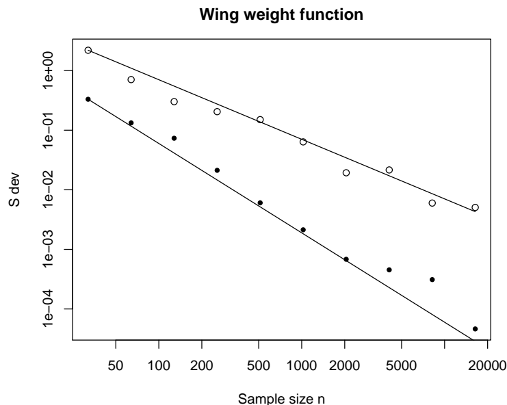
Figure 5: Solid points show standard deviation for scrambled Sobol' estimate \hat{\mu}_{x,1} versus n from R = 10 replicates. A reference line parallel to n^{-3/2} goes through the first solid point. Open points show standard deviation for scrambled Sobol' estimates \hat{\mu}_{x,2} which drop the initial zero. A reference line parallel to n^{-1} goes through the first open point.
