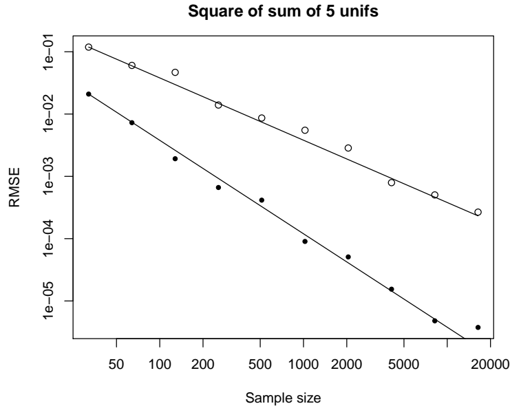
Figure 3: Solid points show RMSE for scrambled Sobol' estimate \hat{\mu}_{x,1} versus n from R = 10 replicates. A reference line parallel to n^{-3/2} goes through the first solid point. Open points show RMSE for scrambled Sobol' estimates \hat{\mu}_{x,2} which drop the initial zero. A reference line parallel to n^{-1} goes through the first open point.
