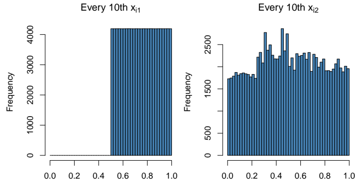
Figure 6: The left panel shows a histogram of every 10 th x_{i_1} from the first 2^{20} Sobol' points. The right panel shows a histogram of every 10 th x_{i_2} from the first 2^{20} Sobol' points.
