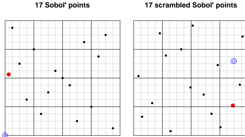
Figure 1: The left panel shows the first 17 Sobol' points in [0, 1]^2 . The initial point at (0, 0) is shown in concentric circles. The 17'th point is shown as a large disk. Solid reference lines partition [0, 1]^2 into 16 congruent squares. Dashed reference lines partition it into 256 congruent squares. The right panel shows a nested uniform scramble of these 17 points.
