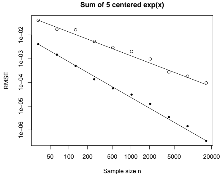
Figure 2: Solid points show RMSE for scrambled Sobol' estimate \hat{\mu}_{x,1} versus n from R = 10 replicates. A reference line parallel to n^{-3/2} goes through the first solid point. Open points show RMSE for scrambled Sobol' estimates \hat{\mu}_{x,2} which drop the initial zero. A reference line parallel to n^{-1} goes through the first open point.
