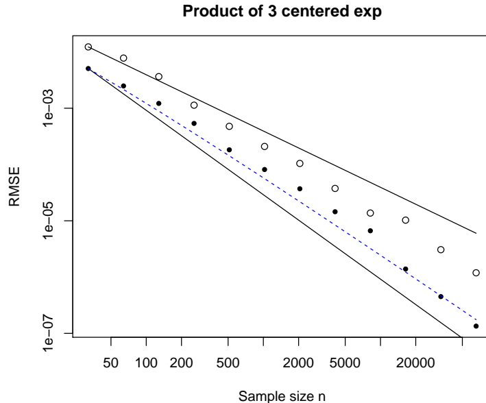
Figure 4: The integrand is a product of 3 centered exponentials. Solid points show RMSE for scrambled Sobol' estimate \hat{\mu}_{\mathbf{x},1} versus n from R = 10 replicates. A reference line parallel to n^{-3/2} goes through the first solid point. Open points show RMSE for scrambled Sobol' estimates \hat{\mu}_{\mathbf{x},2} which drop the initial zero. A reference line parallel to n^{-1} goes through the first open point. A dashed reference line through the first solid point decays as \log(n)/n^{3/2} .
