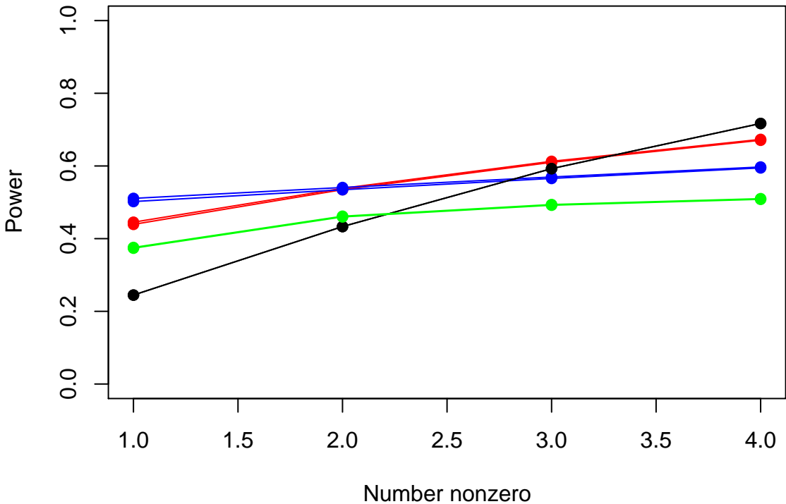
Top Fisher (red) Top LRT (blue) Top Stouffer (black) Stouffer (green) alpha=.05 power=.5
