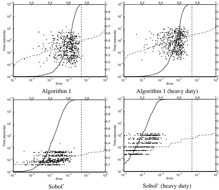
Fig. 5. Execution times and errors for the Asian geometric mean call option for d = 1, 2, 4, 8, 16, 32 and \epsilon = 0.05 .
