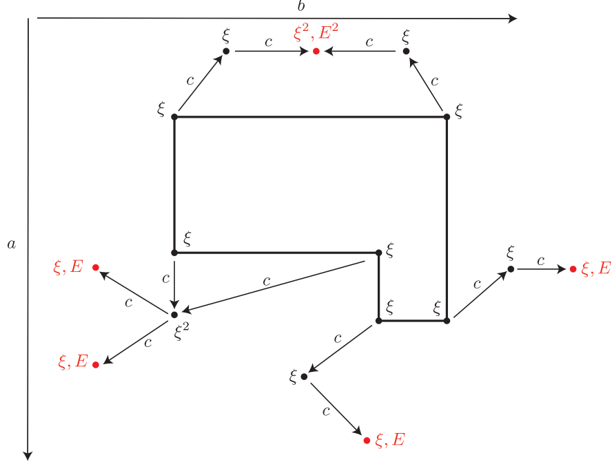
Figure 3: A “spider” with j = 3 and k = 2 , with the “body” in boldface lines and the “legs” as directed paths from the body to the tips (marked in red).
